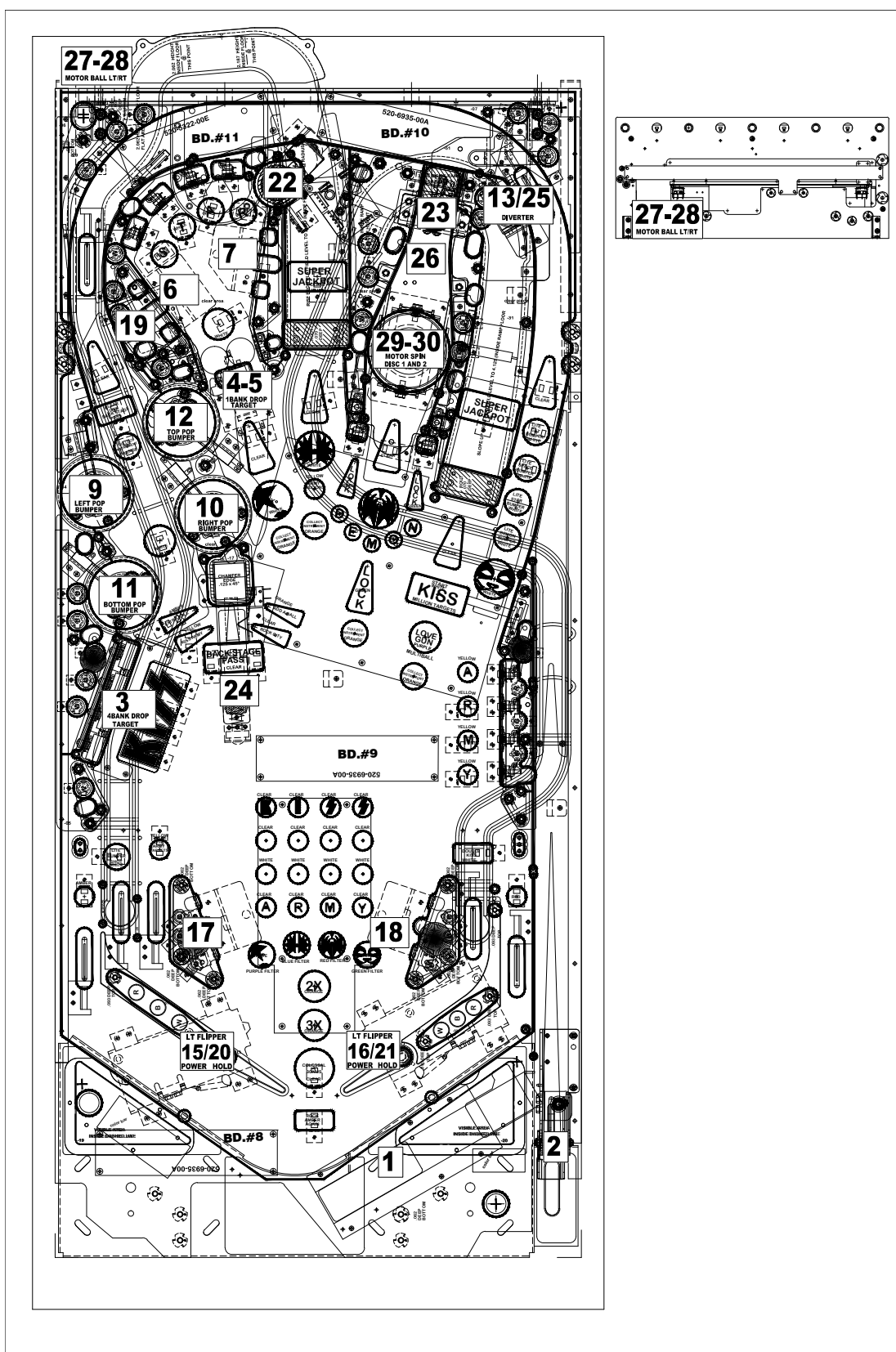
Figure 3.2.1. Playfield top component view
