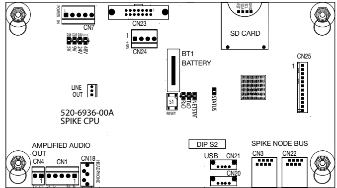
Figure 4.1.1. SPIKE CPU Node connector detail.
